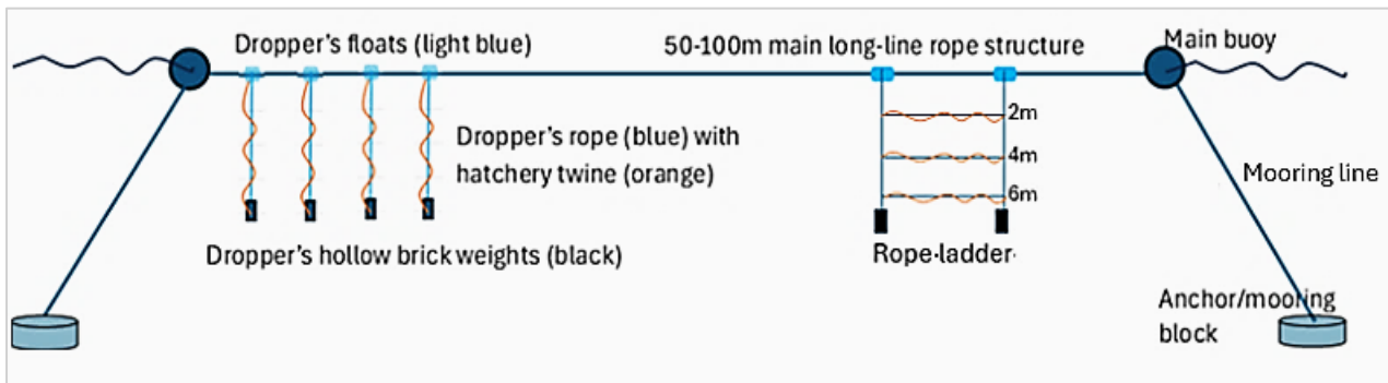
Figure 2. Outline of a rope ladder and rope droppers suspended from the main long-line (Diagram credit: Dr L Botes).
