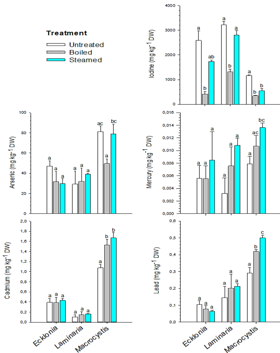
Figure 2. Effects of two blanching methods—2-minutes of boiling or 20-minutes of steaming followed immediately by 5-minutes of rapid cooling in ice water—on the heavy metal (Cd, Pb and Hg), As and I content of E. maxima , M. pyrifera and L. pallida . (Graph credit: Dr BM Macey)
